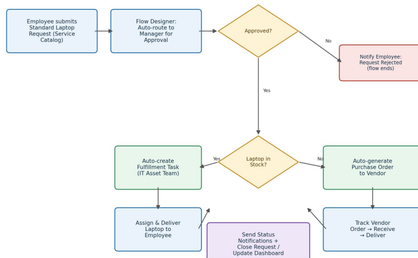
Flow: Automated Standard Laptop Order (IT Procurement - Flow Designer)
